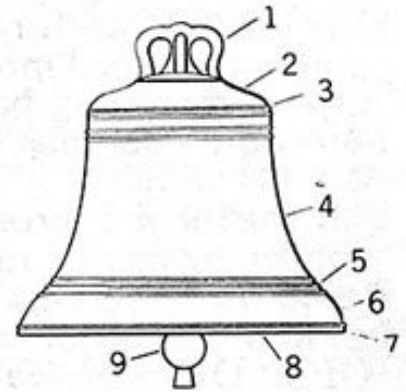
1 crown, 2 head 3 shoulder, 4 waist, 5 bead lines, 6 sound bow, 7 lip 8 mouth, 9 clapper
